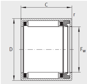
HK..-RS
